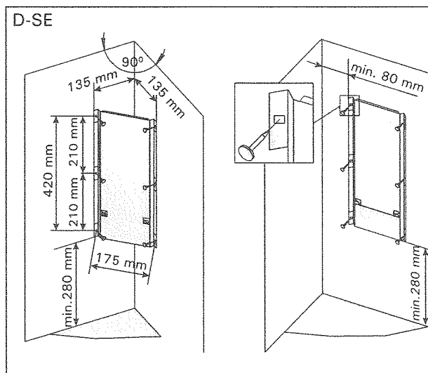
Figure 5. Location of the mounting rack of the heater (D-SE, KV-SE) Abbildung 5. Platz des Montagegestells des Saunaofens (D-SE, KV-SE)
