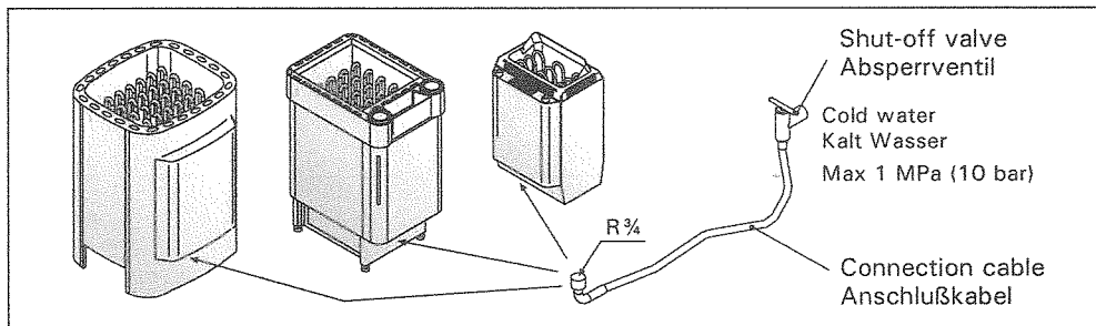
Figure 7. Automatic filling
